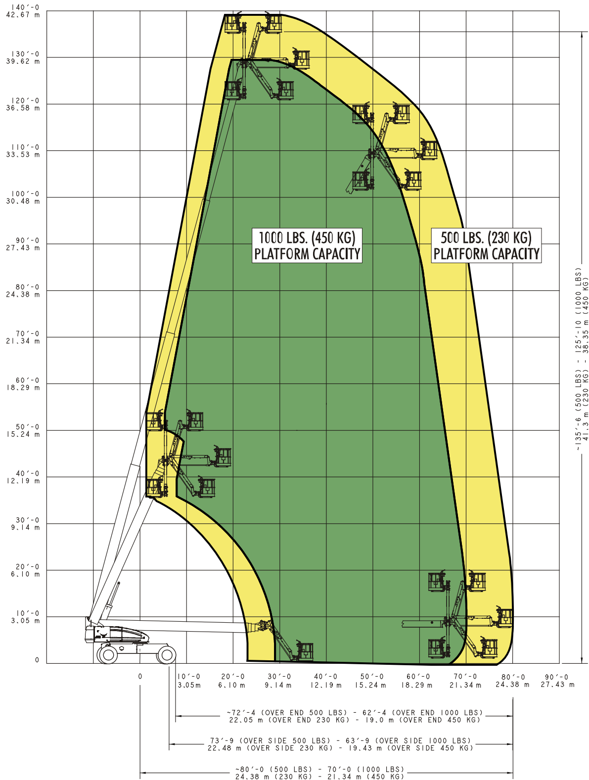
Figure 3-36. 1350SJP Reach Chart
