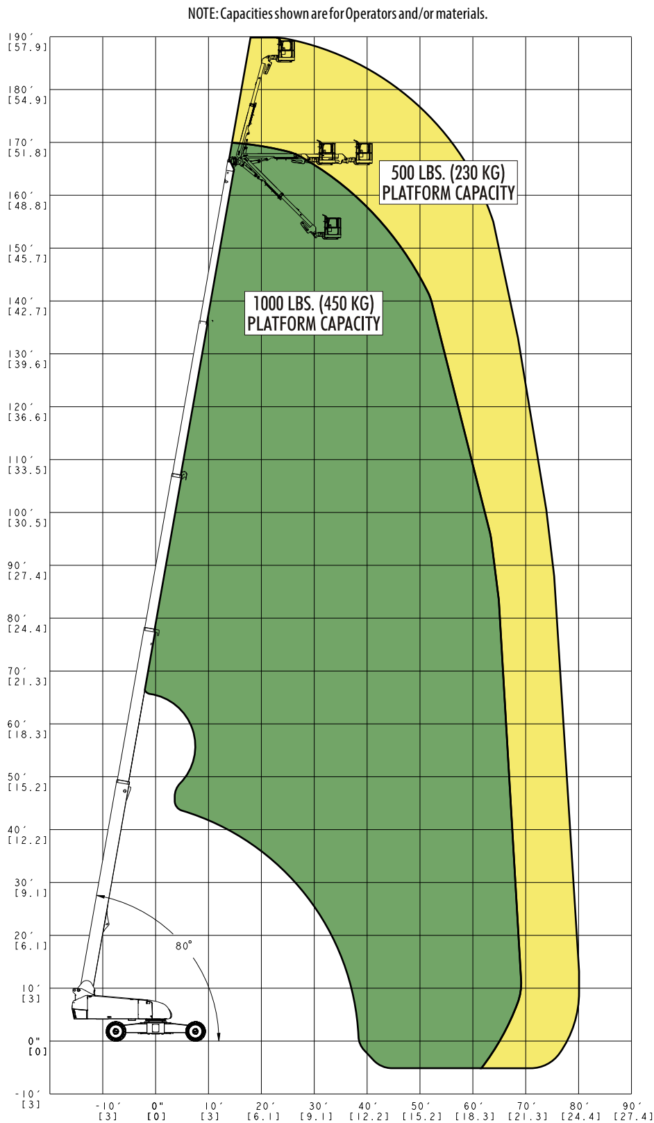
Figure 3-39. 1850SJ Reach Chart
