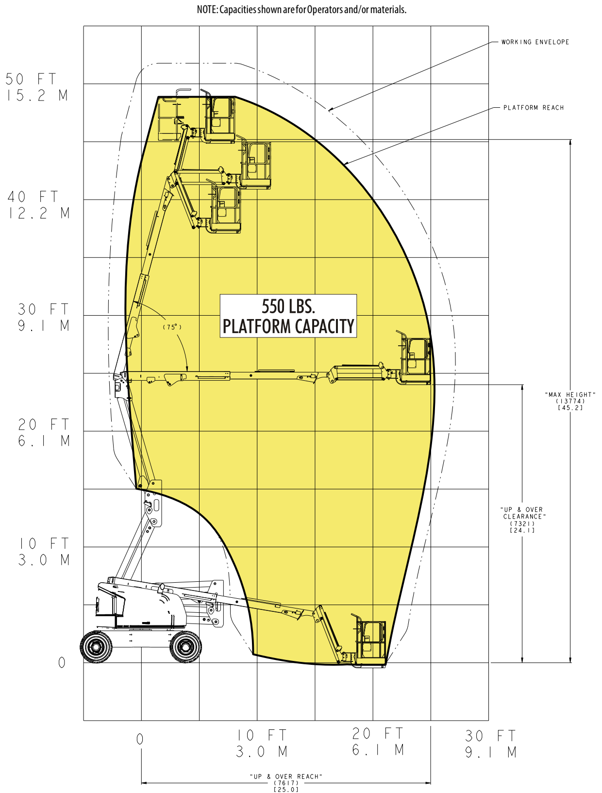
Figure 3-8. 450AJ Reach Chart (SN 03000201991, 1300007279, B00003516 & E300002833 to Present)
